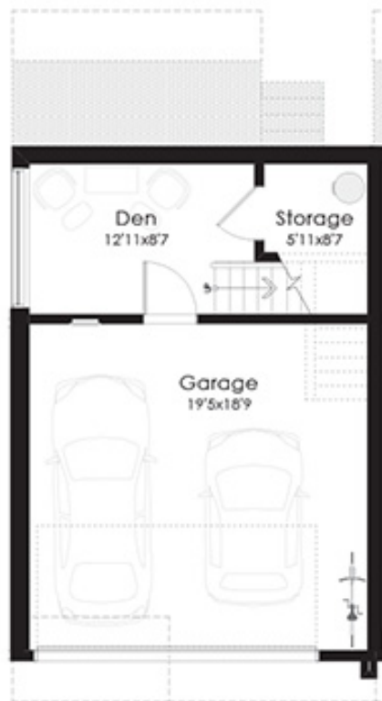
LOWER FLOOR
